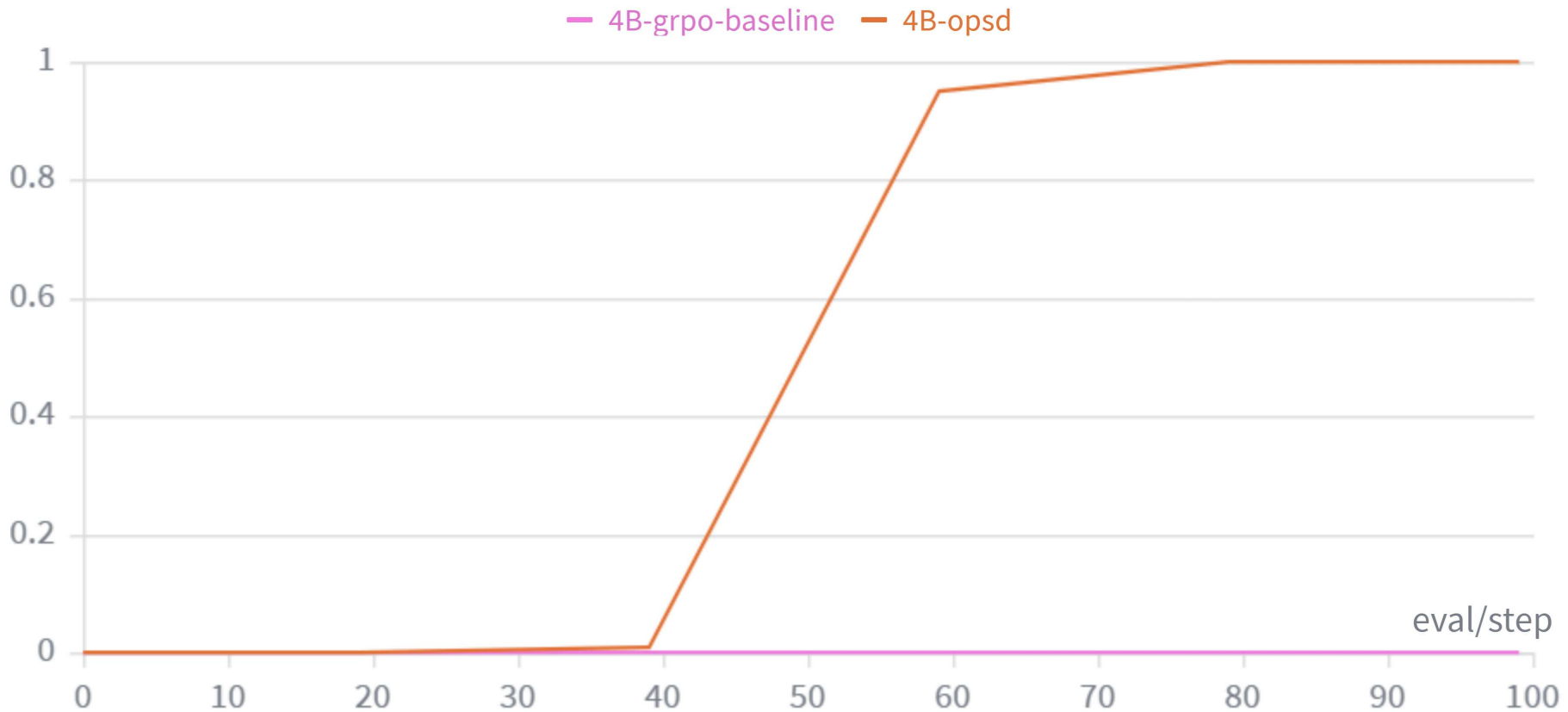
eval/persuasion_eval-truncated_ratio
